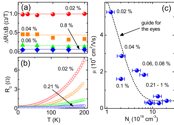
FIG. 3. (a) LMR slopes \Delta R/\Delta B for selected doping levels (0.02%, 0.04%, 0.06%, and 0.8%) as a function of temperature ( T = 4.2\text{--}200\text{ K} ). The slopes are to a good approximation independent on temperature (dotted lines). (b) Zero field resistance R_0(T) , which is plotted for doping levels of 0.02%, 0.04%, 0.08%, and 0.21%, revealing a metallic behavior. (c) Mobilities at T \sim 10\text{ K} of each sample as a function of the scattering center concentration N_i .
